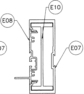
MULLION 'MD2'
