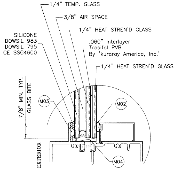
GLAZING DETAIL
