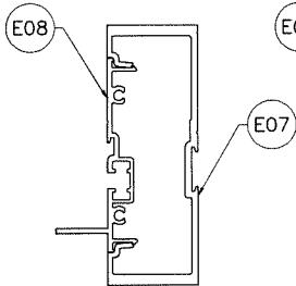
MULLION 'MD1'
