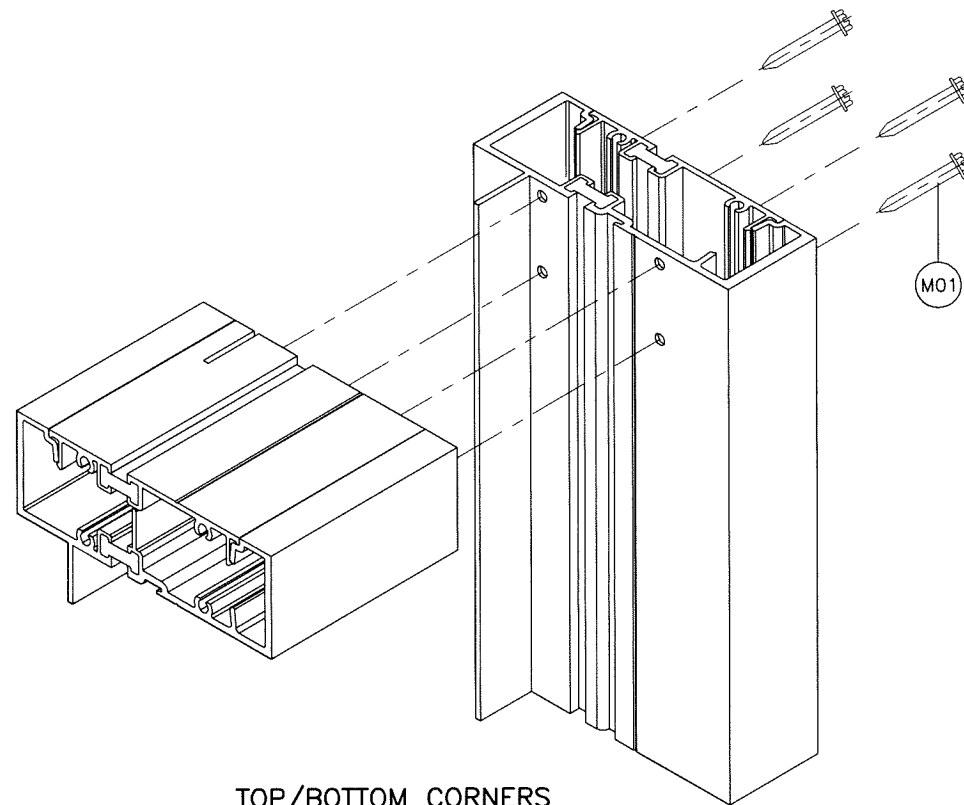
TOP/BOTTOM CORNERS
